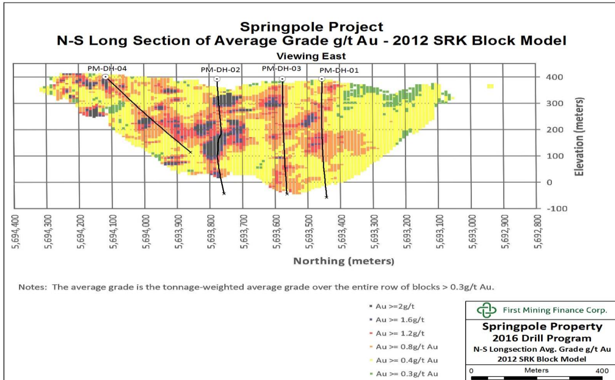
Figure 2. Long Section Map with Grade Blocks
