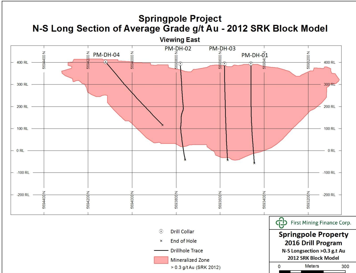
Figure 3. Long Section within Mineralized Zone
